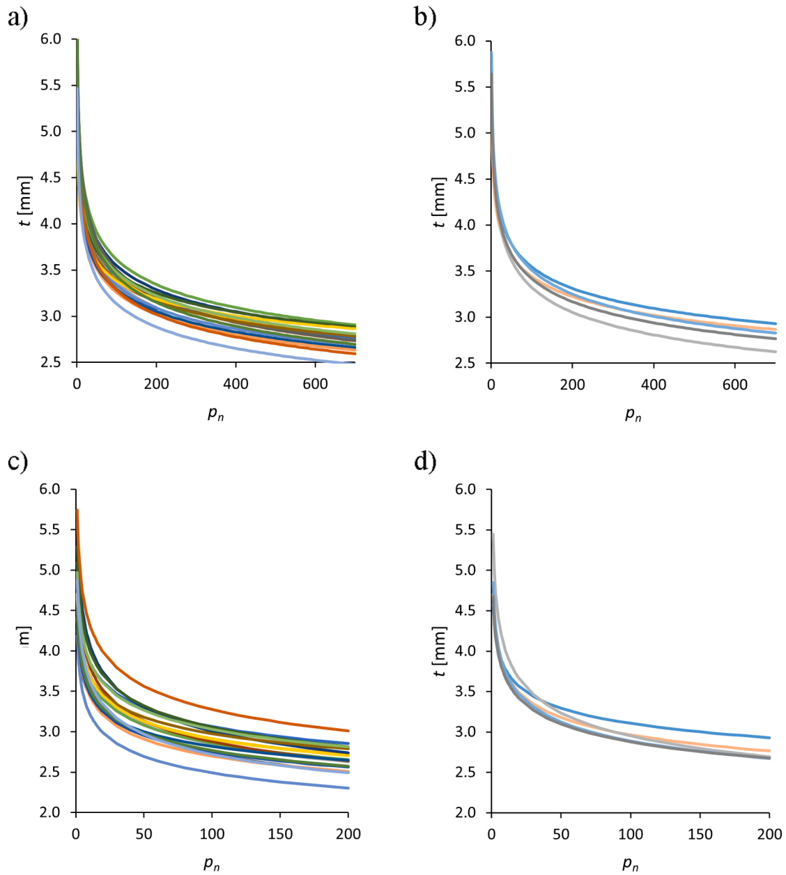
Fig. 9. Fitted wet compaction curve for [thickness measurement source - material] a) [UTM - NCF wet], b) [LVDT/direct - NCF wet], c) [UTM - WOVEN wet] and d) [LVDT/direct - WOVEN wet]. (For interpretation of the references to colour in this figure legend, the reader is referred to the web version of this article.)
