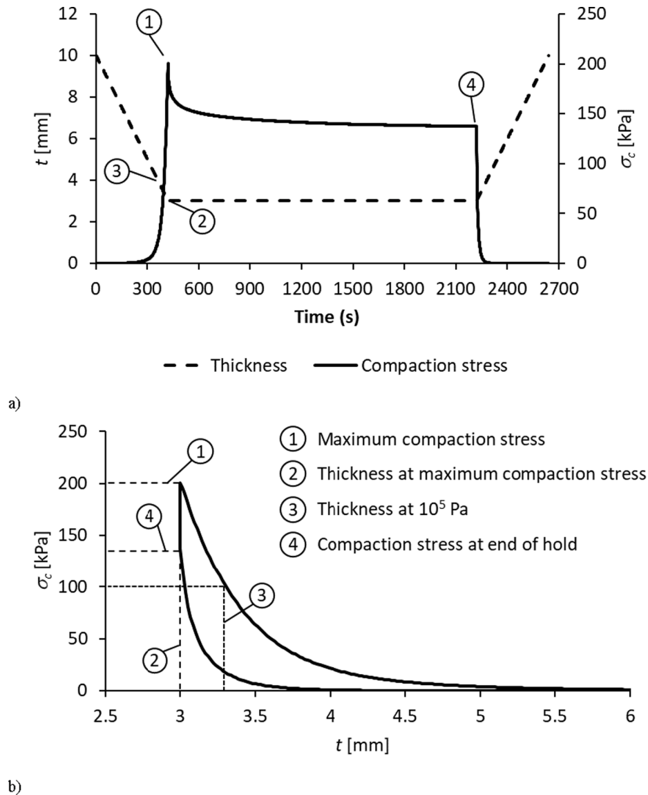
Fig. 2. Data from compaction experiments; a) Representative thickness and compression stress data measured by the participants, b) Data extracted from the thickness – compaction stress curve.
