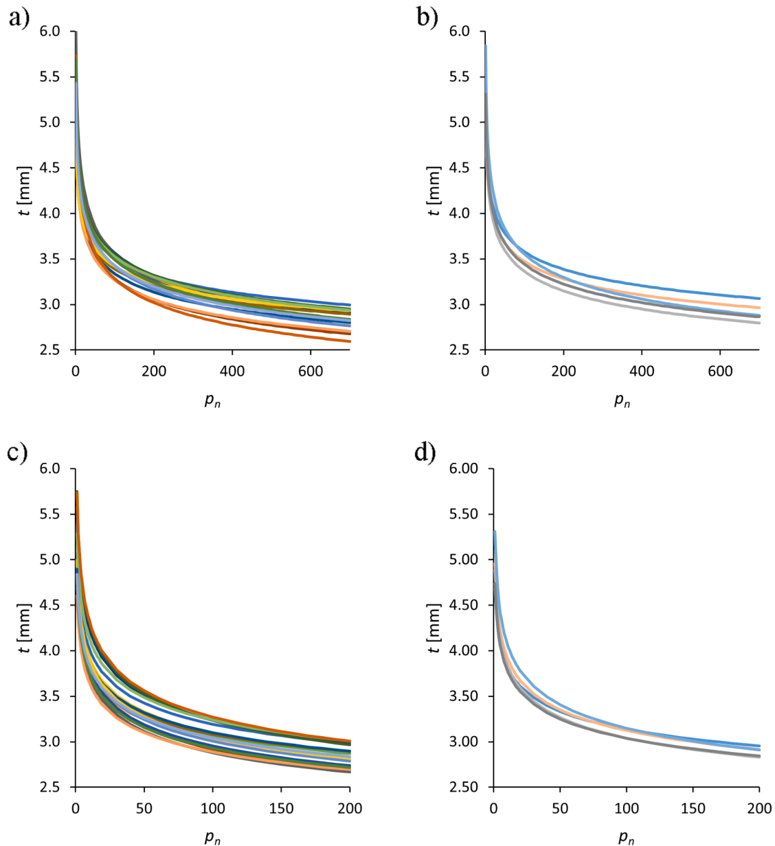
Fig. 8. Fitted dry compaction curve for [thickness measurement source - material] a) [UTM - NCF dry], b) [LVDT/direct - NCF dry], c) [UTM - WOVEN dry] and d) [LVDT/direct - WOVEN dry]. (For interpretation of the references to colour in this figure legend, the reader is referred to the web version of this article.)
