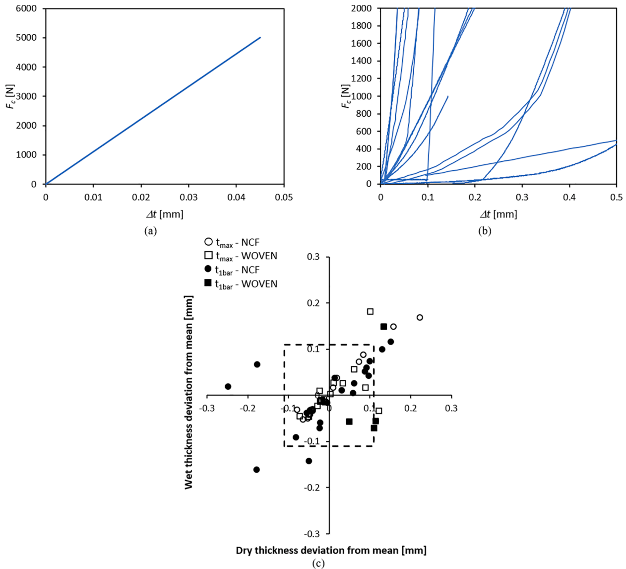
Fig. 3. Machine compliance characterisation; a) Example of a compliance curve for a compression plate set-up on a universal testing machine; compaction force, F_c , is a linear function of apparent cross-head displacement, \Delta t . b) Compliance curves measured by different participants show a wide variety of dependencies of F_c on \Delta t . c) Specimen thickness (maximum and at 10^5 Pa of pressure) deviation from mean for dry and wet conditions compared to the average compliance reported by the participants. The dotted line box represents the average compliance \Delta t = 0.22 mm for an average compaction load F_c = 2700 N. (For interpretation of the references to colour in this figure legend, the reader is referred to the web version of this article.)
