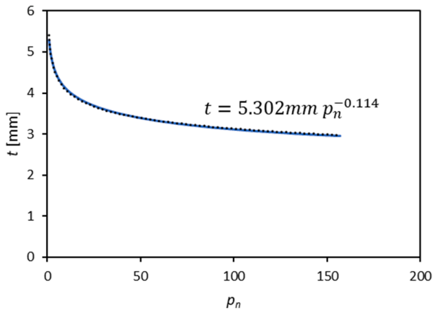
Fig. 7. Specimen thickness, t , as a function of normalised compaction pressure, p_n ; example of processed data allowing a power-curve to be fitted with R^2 = 0.999 . (For interpretation of the references to colour in this figure legend, the reader is referred to the web version of this article.)
