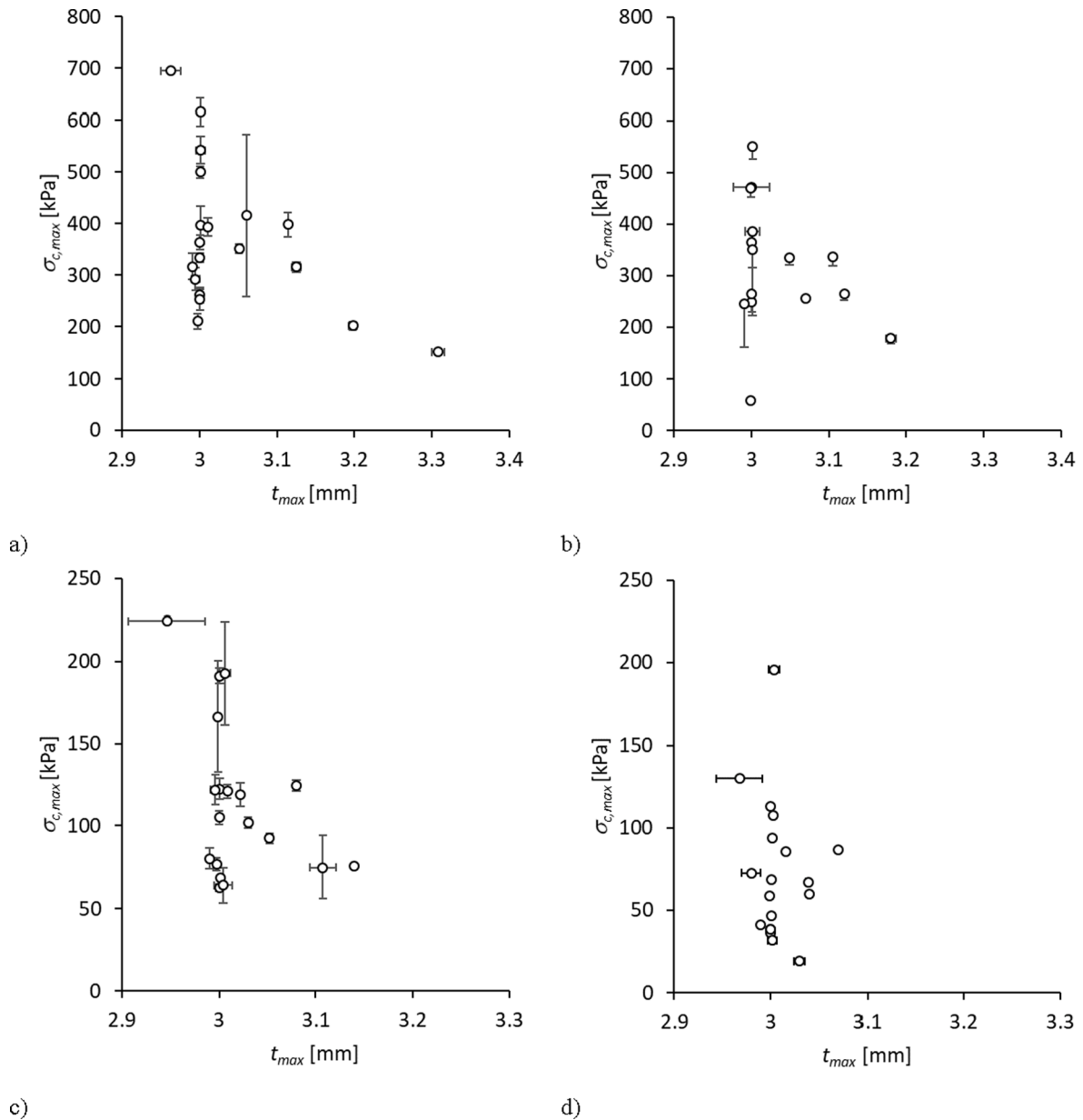
Fig. 5. Maximum compaction stress, \sigma_{c,max} , and corresponding measured thickness, t_{max} , obtained with UTM thickness measurement for a) NCF dry, b) NCF wet, c) WOVEN dry and d) WOVEN wet.
