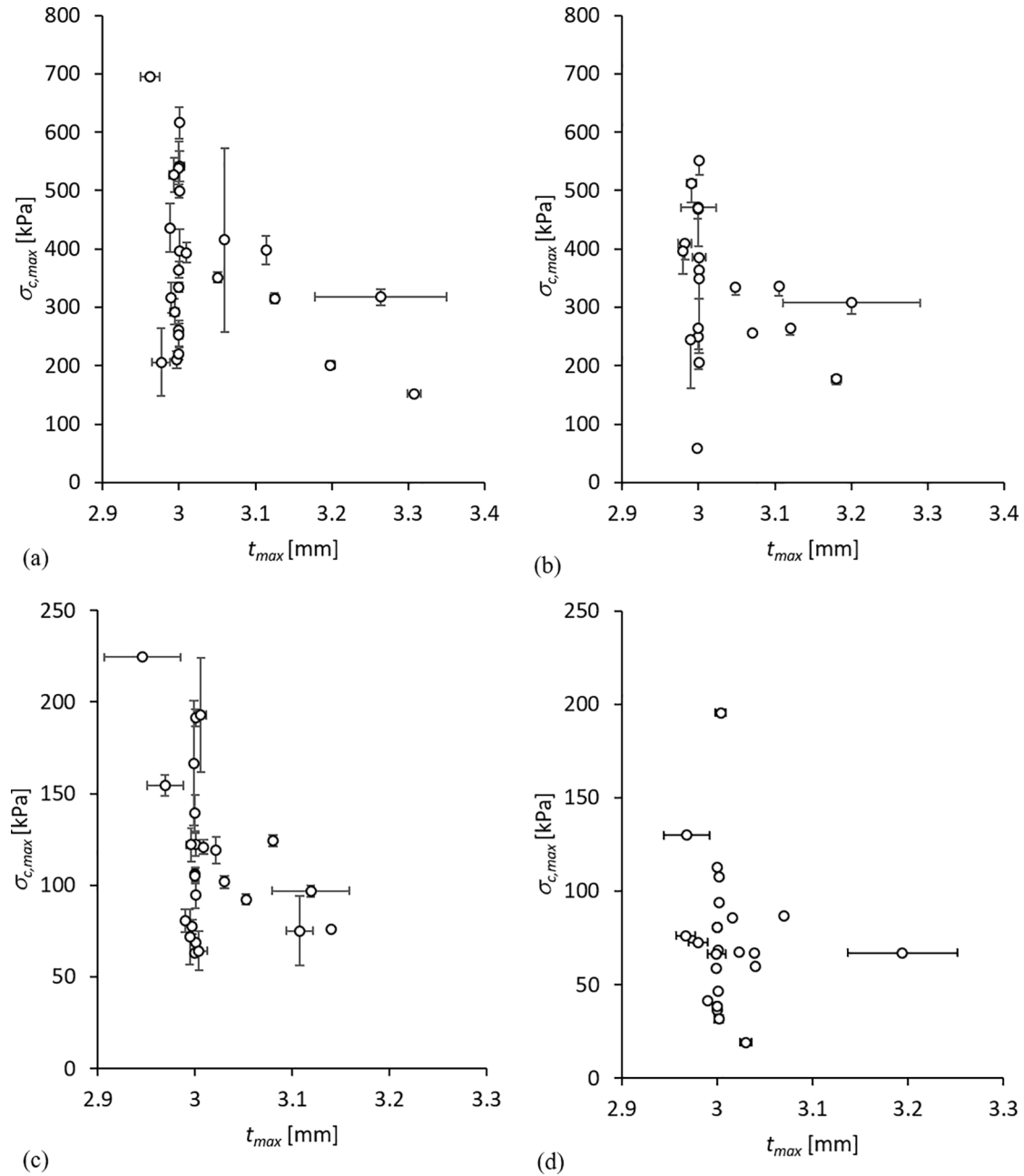
Fig. 4. Maximum compaction stress, \sigma_{c,max} , as a function of corresponding measured thickness, t_{max} , for all participants a) NCF dry, b) NCF wet, c) WOVEN dry and d) WOVEN wet.
