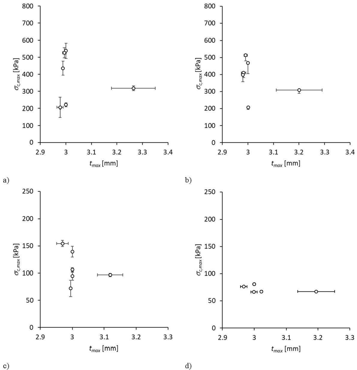
Fig. 6. Maximum compaction stress, \sigma_{c,max} , and corresponding measured thickness, t_{max} , obtained with LVDT or other direct thickness measurement for a) NCF dry, b) WOVEN wet, c) NCF dry and d) WOVEN wet.
