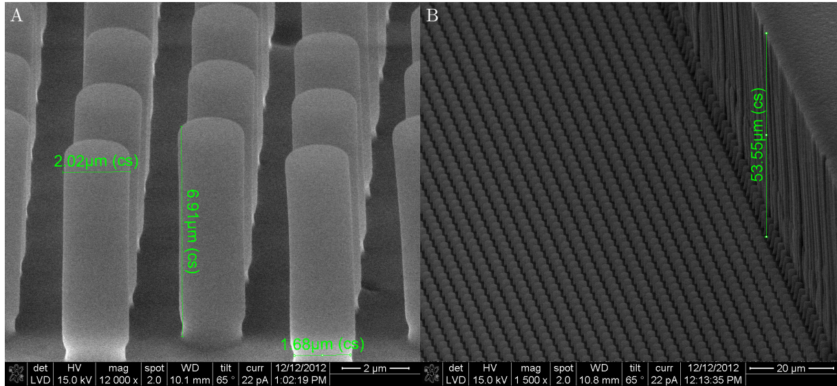
Figure 11: Electron micrographs of a pillar array. A. Dimensions of a pillar are shown. B. The spacer of about 50 \mu\text{m} high keeps some space between the pillars and the microscope slide.
