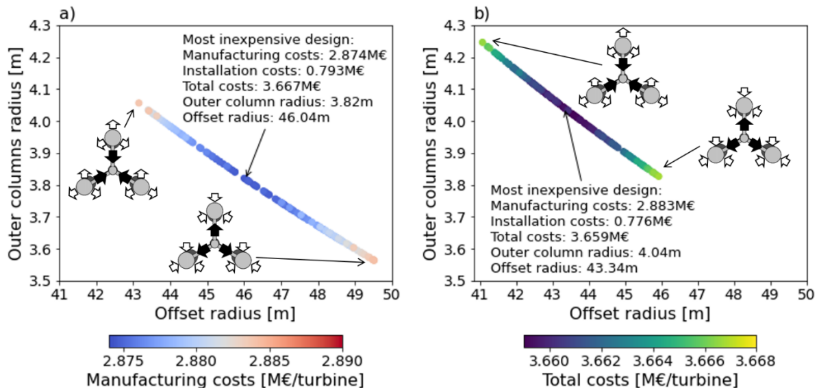
Figure 1: Cost of the 150 best semi-submersible designs obtained from the multi-start optimisation of the floating semi-submersible. a) objective limited to fabrication costs and b) also including installation costs
